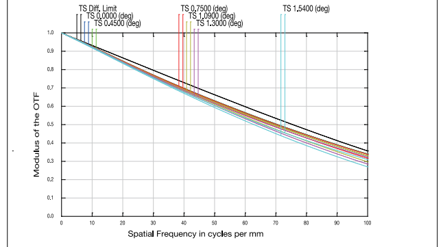
MTF 1" (900~1700nm 100lp/mm)
