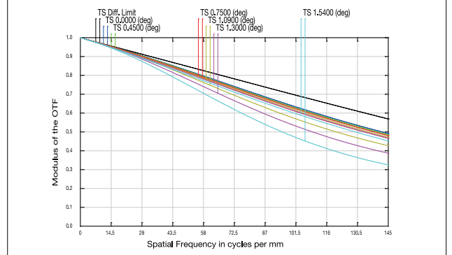
MTF 1" (400~1700nm 100lp/mm)
