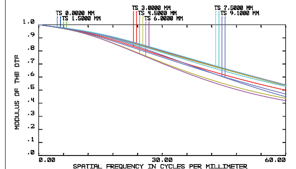
MTF
